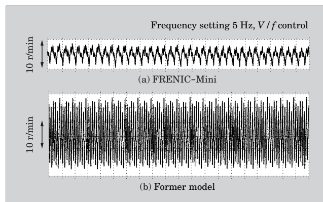
Fig.6 Dynamic characteristics of motor instability at low speed
